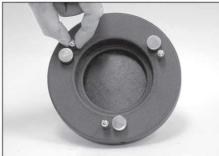
Figure 13. The three thin thumbscrews that lock the primary mirror in place must first be loosened before any adjustments can be made.
