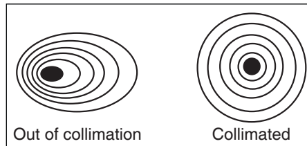
Figure 15. A star test will determine if the telescope's optics are properly collimated. An unfocused view of a bright star through the eyepiece should
