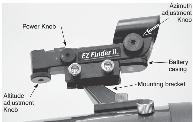
Figure 6. The EZ Finder II reflex sight.
